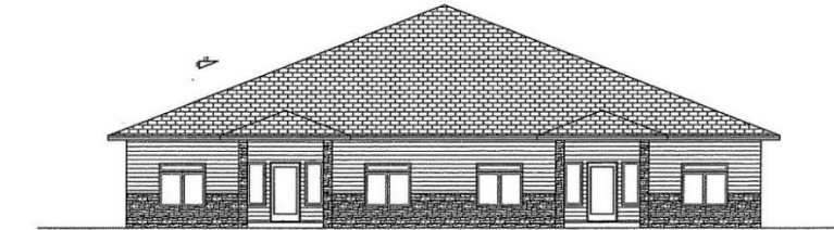
FRONT ELEVATION SCALE: 1/4\"/>
